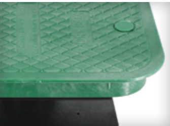
T-LIP LID DESIGN The T-Lip lid design keeps dirt out, while the snap fit and bolt retention for security.
